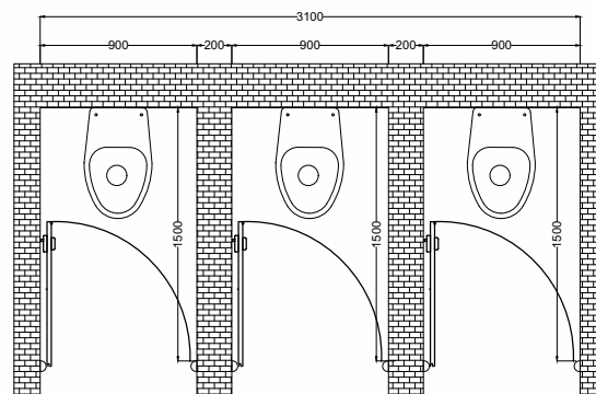
Top View (EU)
