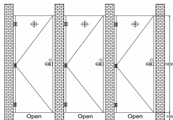
Front View (EU)
